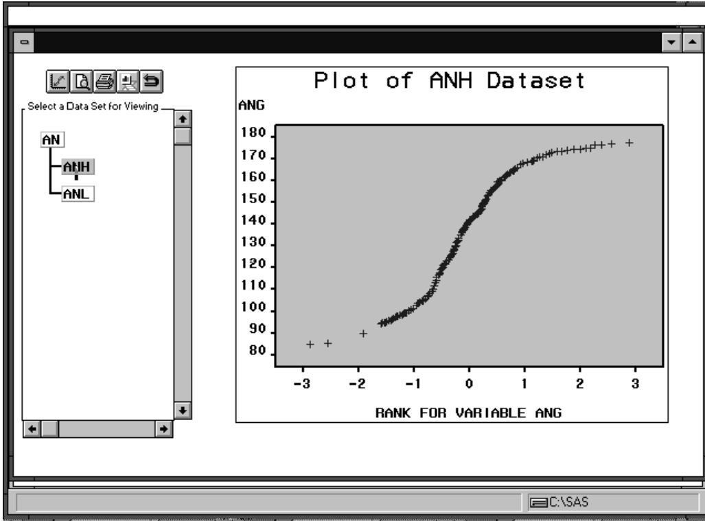
Figure 3 - Classification screen
